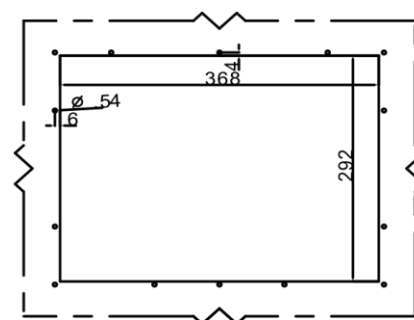
IP65 CUT OUT
